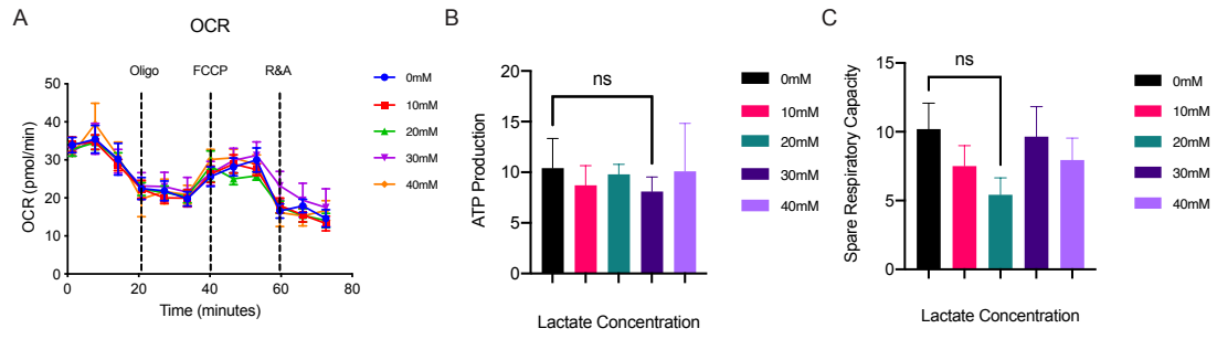
Figure S1 Effects of lactate on oxidative phosphorylation levels of A253. (A) A Seahorse assay was performed to measure OCR in A253 cells under different concentrations of lactate. (B, C) ATP production and spare respiratory capacity of A253 cells in a high-lactate environment.
