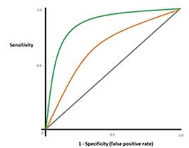
Diagnostic Performance
