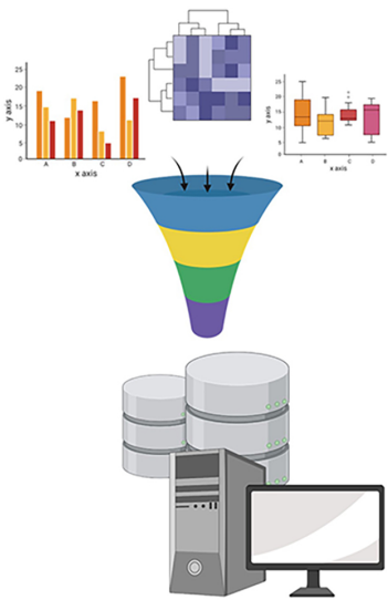
Data Mining
